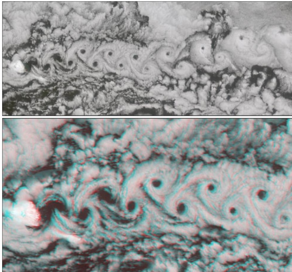
Figure 2: Photographs of von Karman streets in clouds (see also ref. [1])
