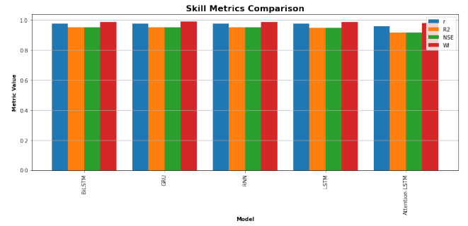
Figure 9. Comparison of skill metrics ( r , R^2 , NSE, and WI) for different deep learning models.
