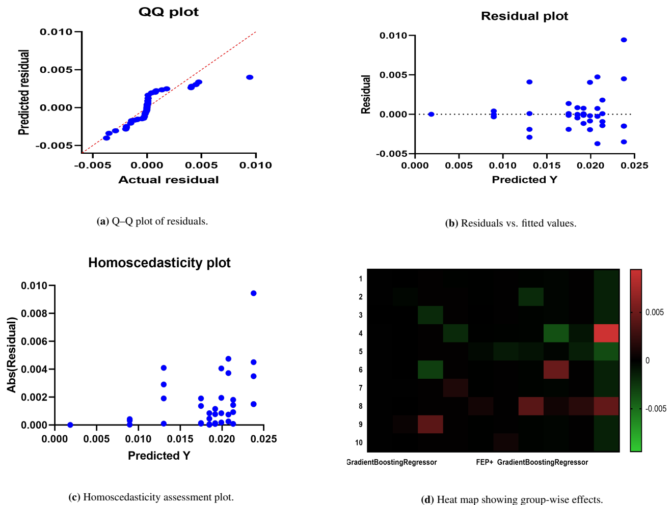
Figure 13. Diagnostic plots for evaluating residual assumptions in one-way ANOVA, including normality (a), homoscedasticity (b–c), and group effect visualization (d).
