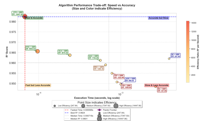
Figure 17. Algorithm performance deviation from mean values of execution time and R^2 score.
