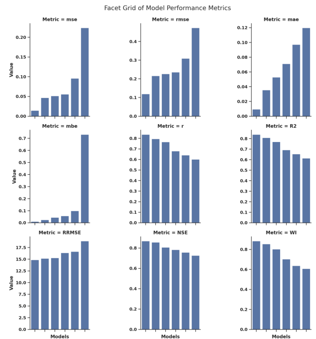
Figure 6. Facet grid of model performance across regression error and agreement metrics. While these measures capture predictive accuracy of timing intervals, subsequent sections introduce verification metrics (EER, FAR, FRR, AUC) to establish direct links with authentication performance.
