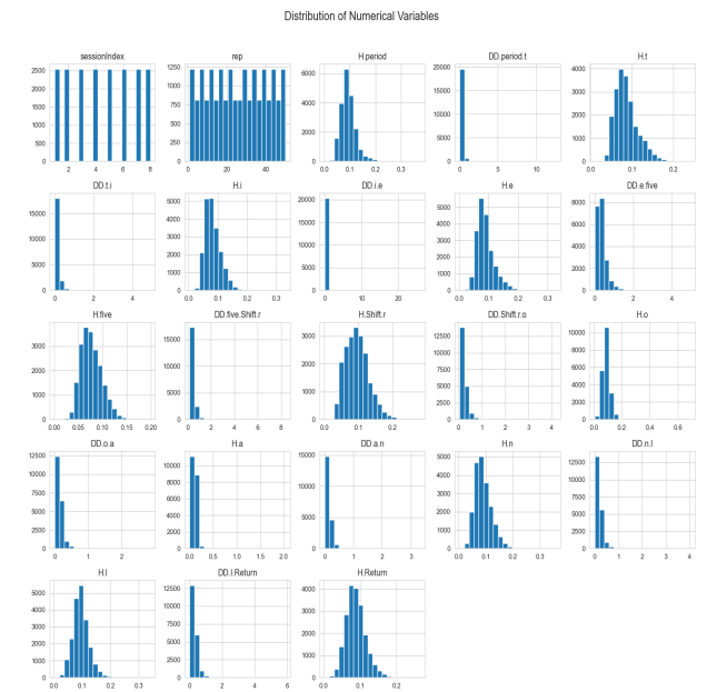
Figure 3. Histograms of the Distribution of Numerical Features
