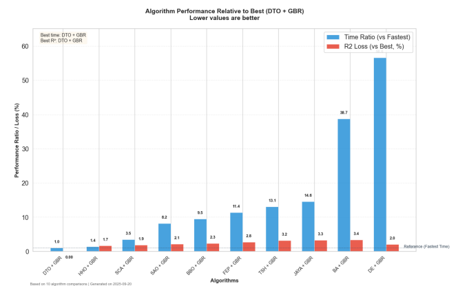
Figure 18. Efficiency ranking by R^2 /Execution Time ratio.
