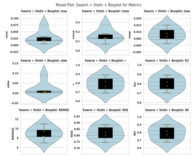
Figure 7. Mixed violin, swarm, and box plots representing the distribution of post-optimization model evaluation metrics.
