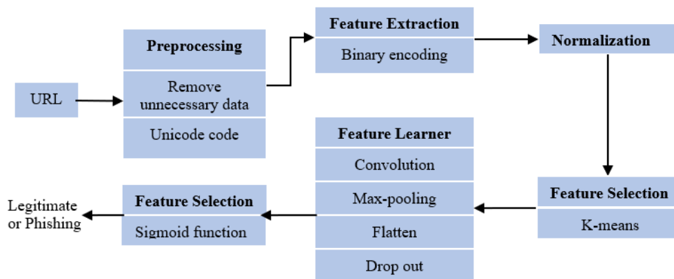
Figure 3. FSRE-K-means-CNN
