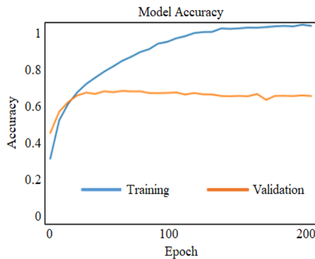
Figure 11. Model Accuracy
