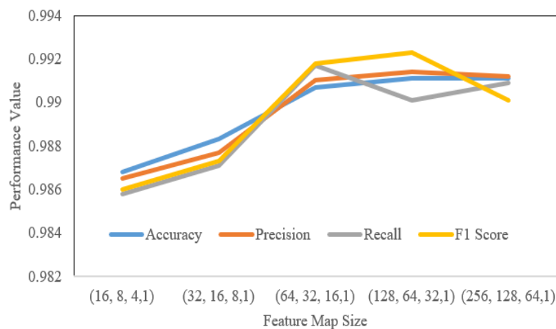
Figure 9. Explore a range of feature map sizes and assess their performance by measuring relevant metrics
