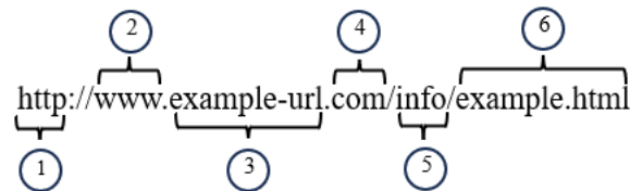
Figure 4. URL components
