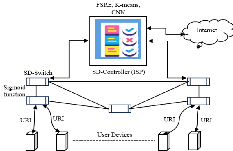
Figure 2. Proposed Model
