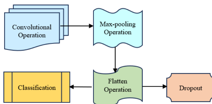
Figure 5. Feature Learner
