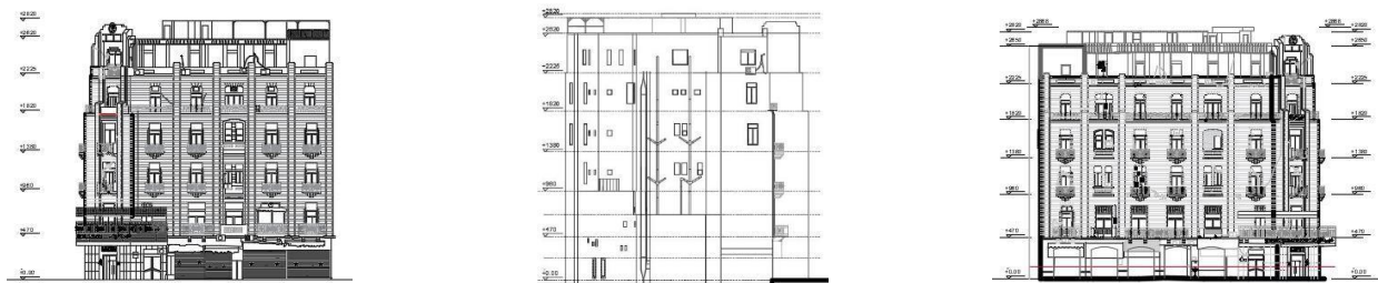
Figure 3. Elevations of the building.
