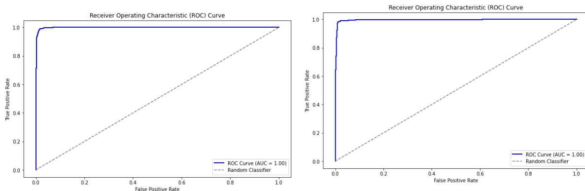
Xception with Fuzzy
