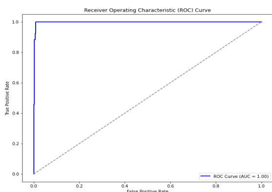
AlexNet
