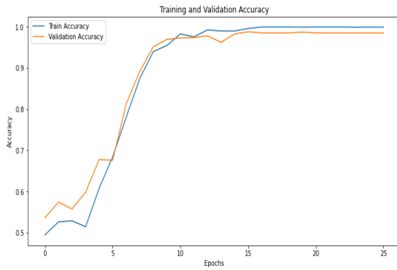
AlexNet
