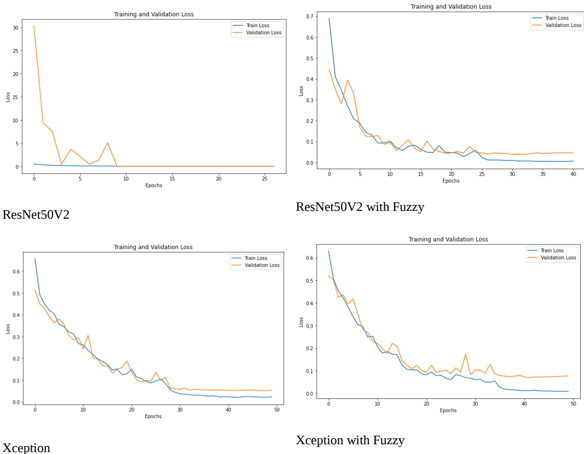
Figure 4. The training and validation loss curves
