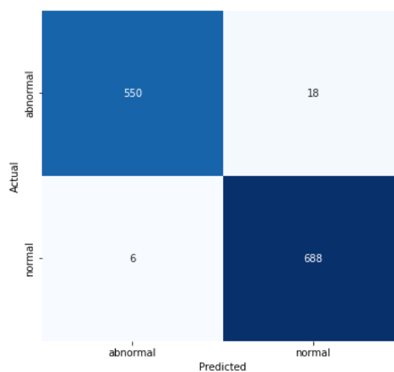
Xception with Fuzzy
