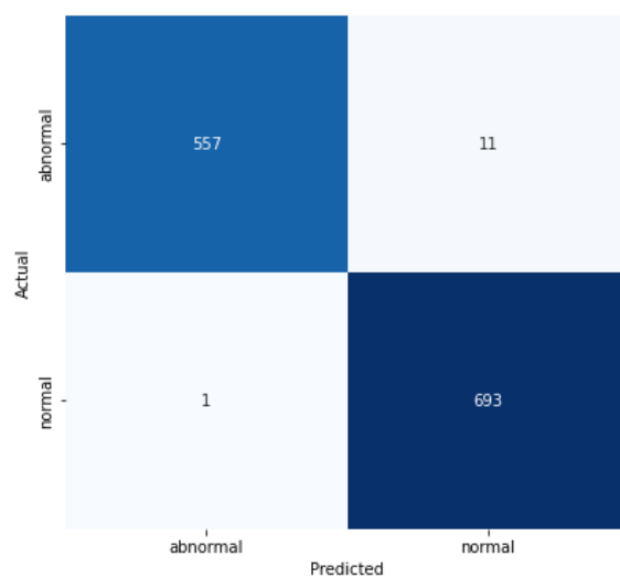
ResNet50V2 with Fuzzy
