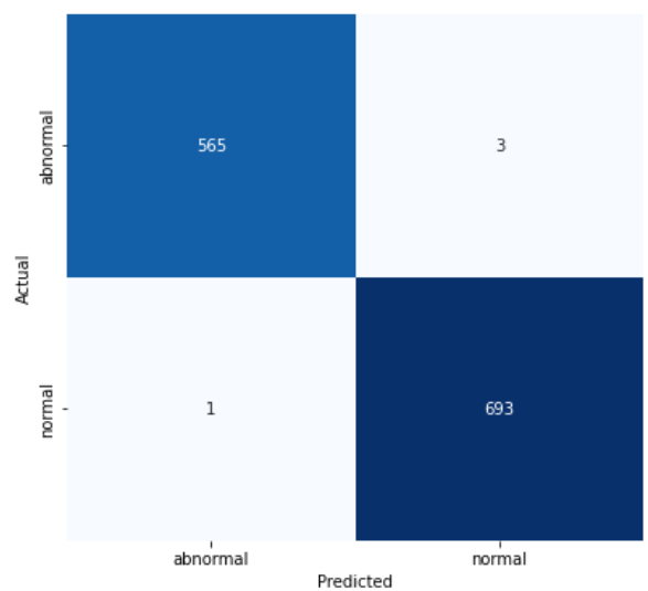
ResNet50V2
