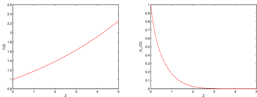
Figure 3: Estimation of the Lyapunov function \|L^*(3)\| and F(3)
