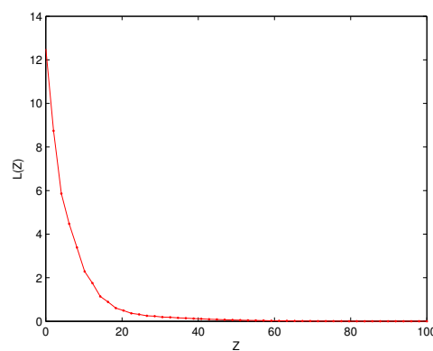
Figure 8: Estimation of the Lyapunov function L(3)
