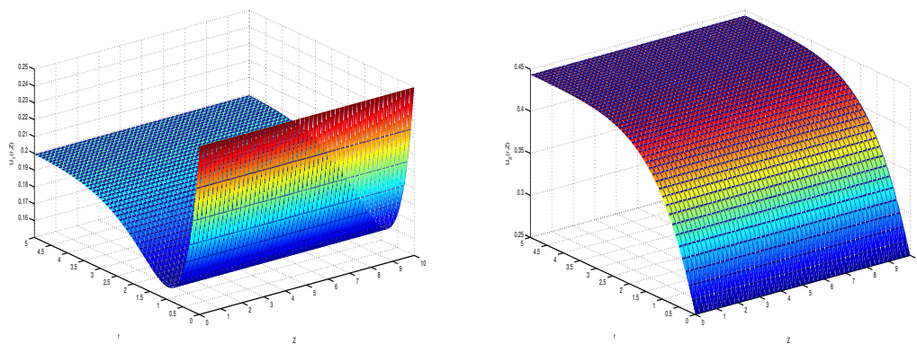
Figure 1: Dynamics behavior of solutions U_1(\tau, 3) and U_2(\tau, 3)
