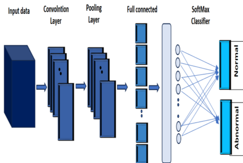
Figure 2. CNN Architecture
