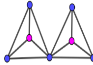
Figure 4: Pyrosilicate
