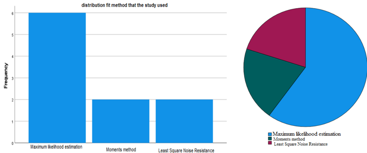
Figure 1. Distribution fit method that the study used
