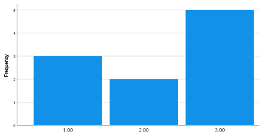
Figure 3. Number of parameters of the Frechette distribution
