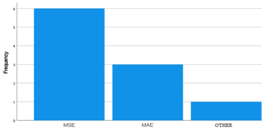
Figure 4. Any measure of error is minimized
