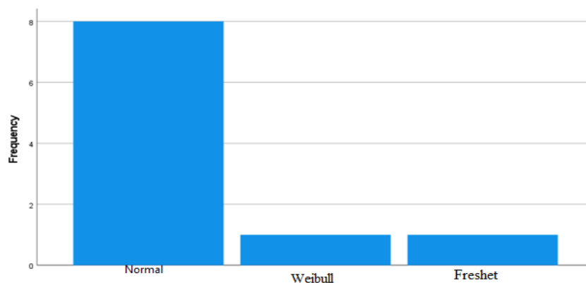
Figure 2. For any distribution the coefficients were estimated
