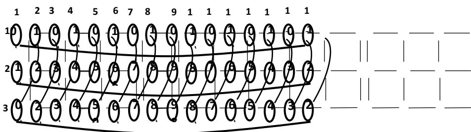
Figure 1. a 2-conversion set on C_3 \times C_{16} starting with S_0 of cardinality 9.
