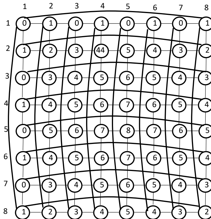
Figure 2. c_2(C_8 \times C_8) \leq 7 .
