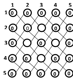
Figure 5. 3-unconvertable U_3 on P_5 \times P_5 .
