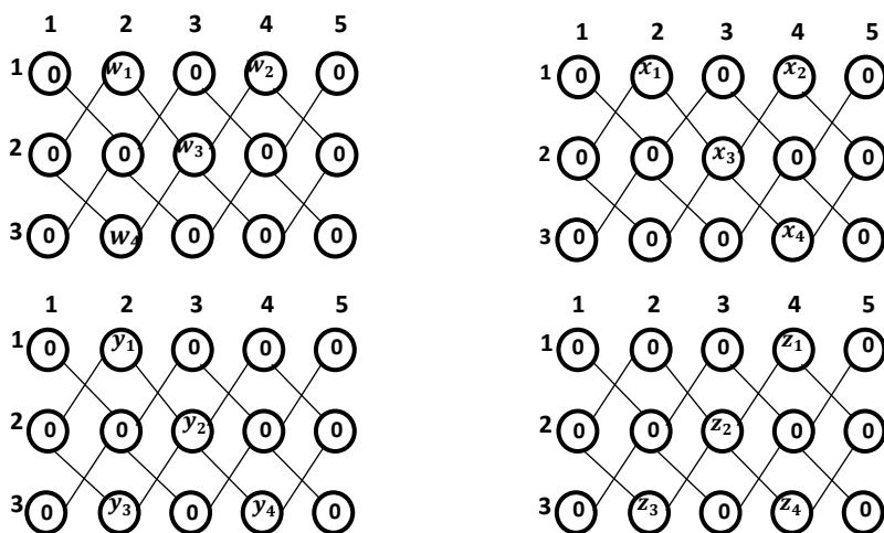
Figure 3. 2-unconvertible W_3, X_3, Y_3 and Z_3 on P_3 \times P_5 .
