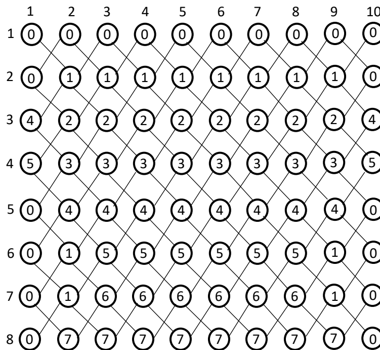
Figure 4. c_2(P_8 \times P_{10}) \leq 20 .
