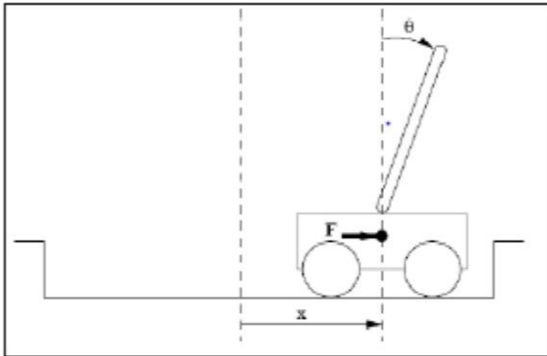
Figure 1. CartPole-v1 environment
