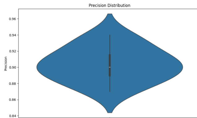
Fig. 7. Precision Distribution
