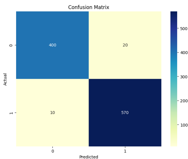
Fig. 11. Confusion Matrix
