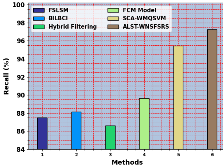
Figure 4: Recall_i outcome of ALST-WNSFSRS technique with existing methods
