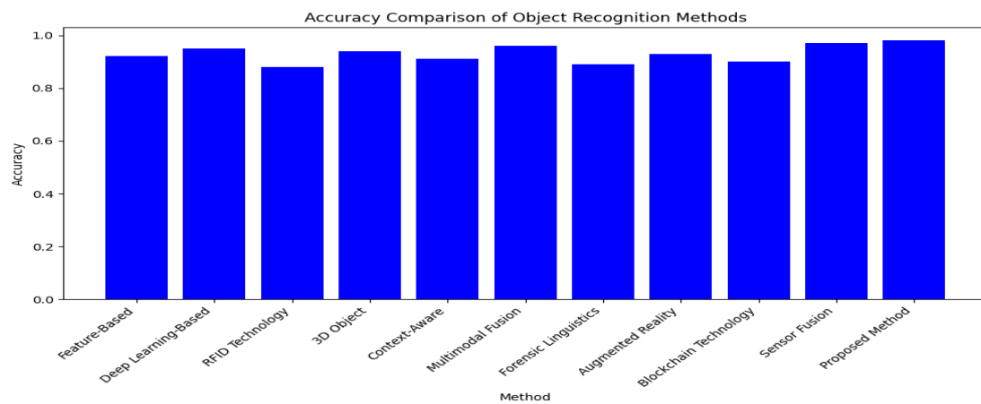
Figure 6: Accuracy Comparison
