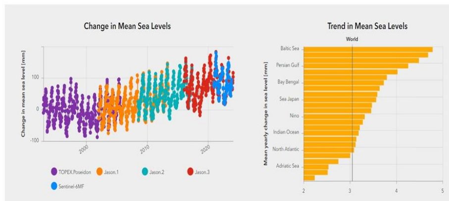
Figure 4: Mean sea level change globally [30]
