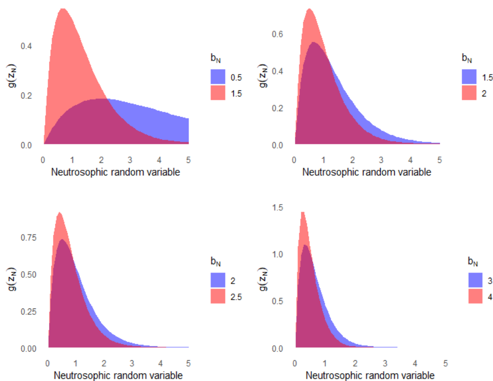
Figure 1: Pdf plot of the proposed distribution with different values of neutrosophic parameter
