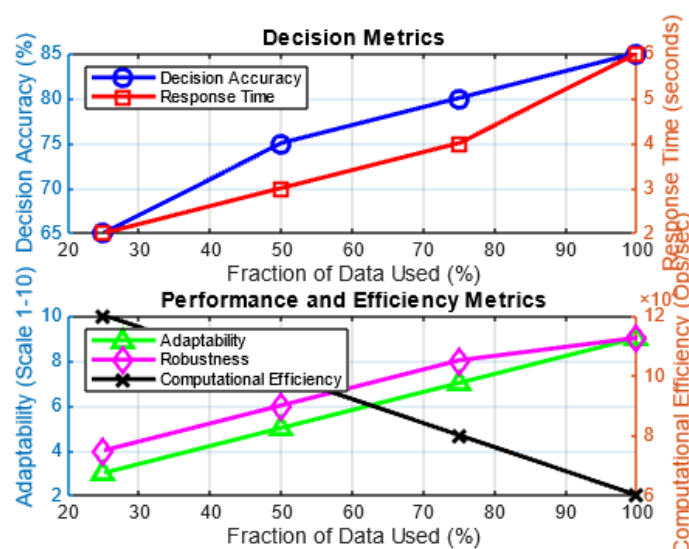
Figure 2: Trend Analysis of Model Performance Metrics by Data Utilization Proportions
