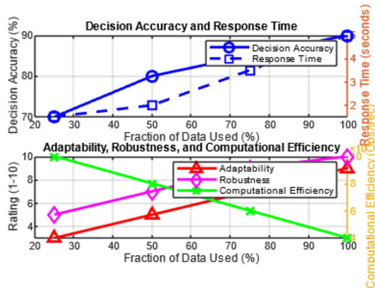
Figure 1: Dynamic Performance Metrics Across Data Utilization Spectrum
