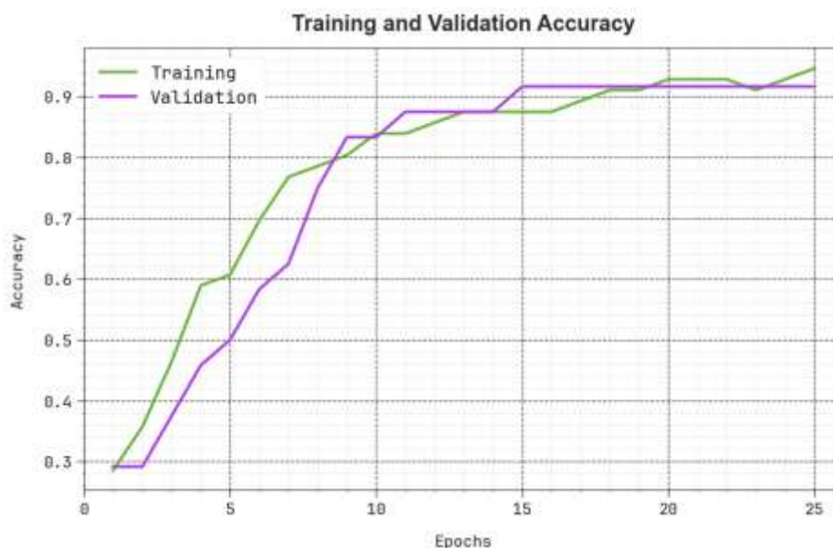
Figure 7: Accu_y curve of the NTOPSIS-TCIE technique
