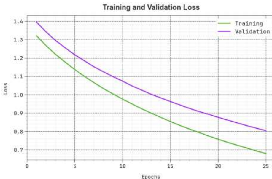
Figure 8: Loss curve of the NTOPSIS-TCIE technique
