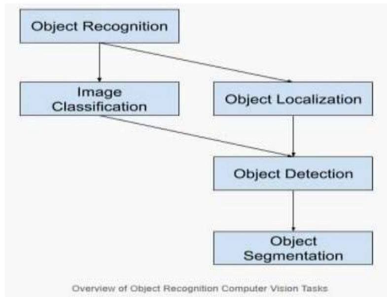
Figure 1: Proposed System
