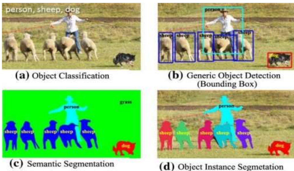
Figure 2: Object classification
