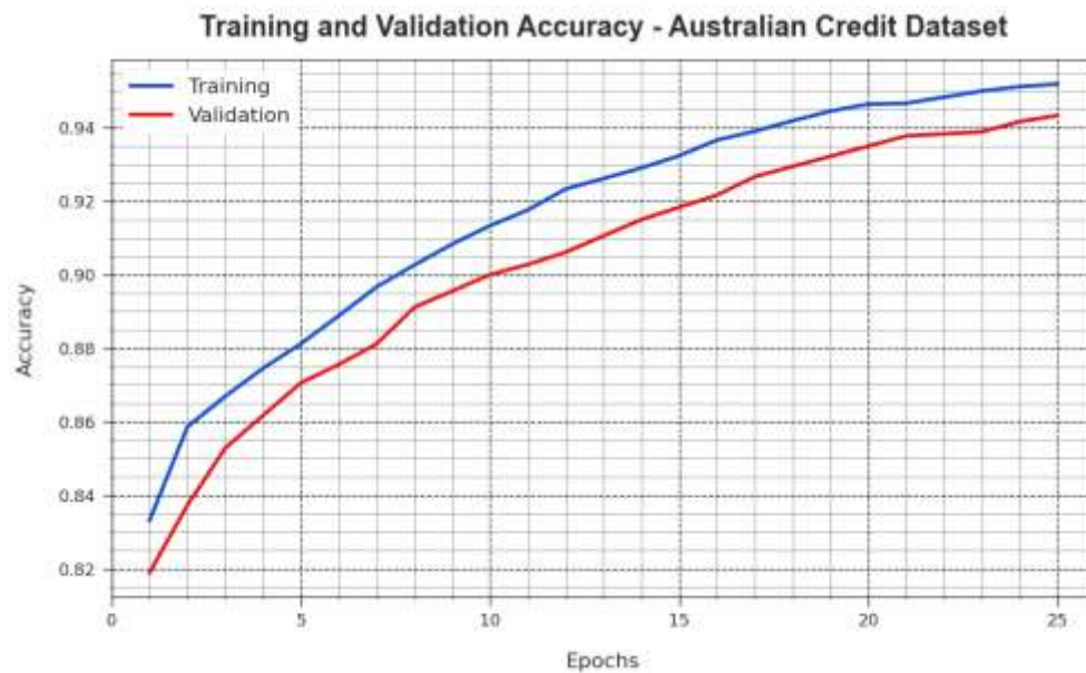
Figure 7: Accu_y curve of OFPSVNS-FCPGF technique under Australian Credit database
