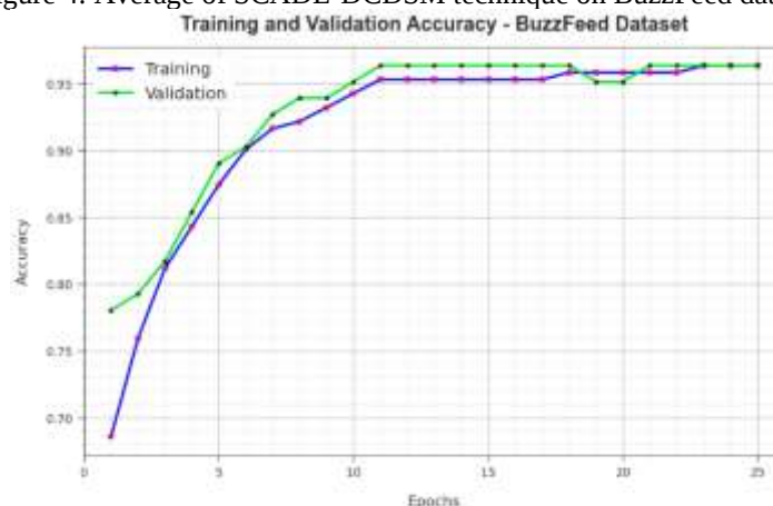
Figure 5: Accu_y curve of SCADL-DCDSM technique on BuzzFeed dataset
