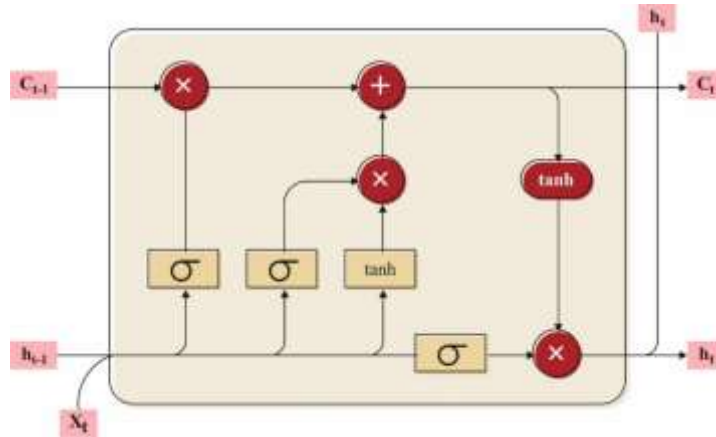
Figure 2: LSTM architecture
