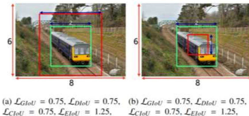
Figure 4: The situation of CIoU failure
