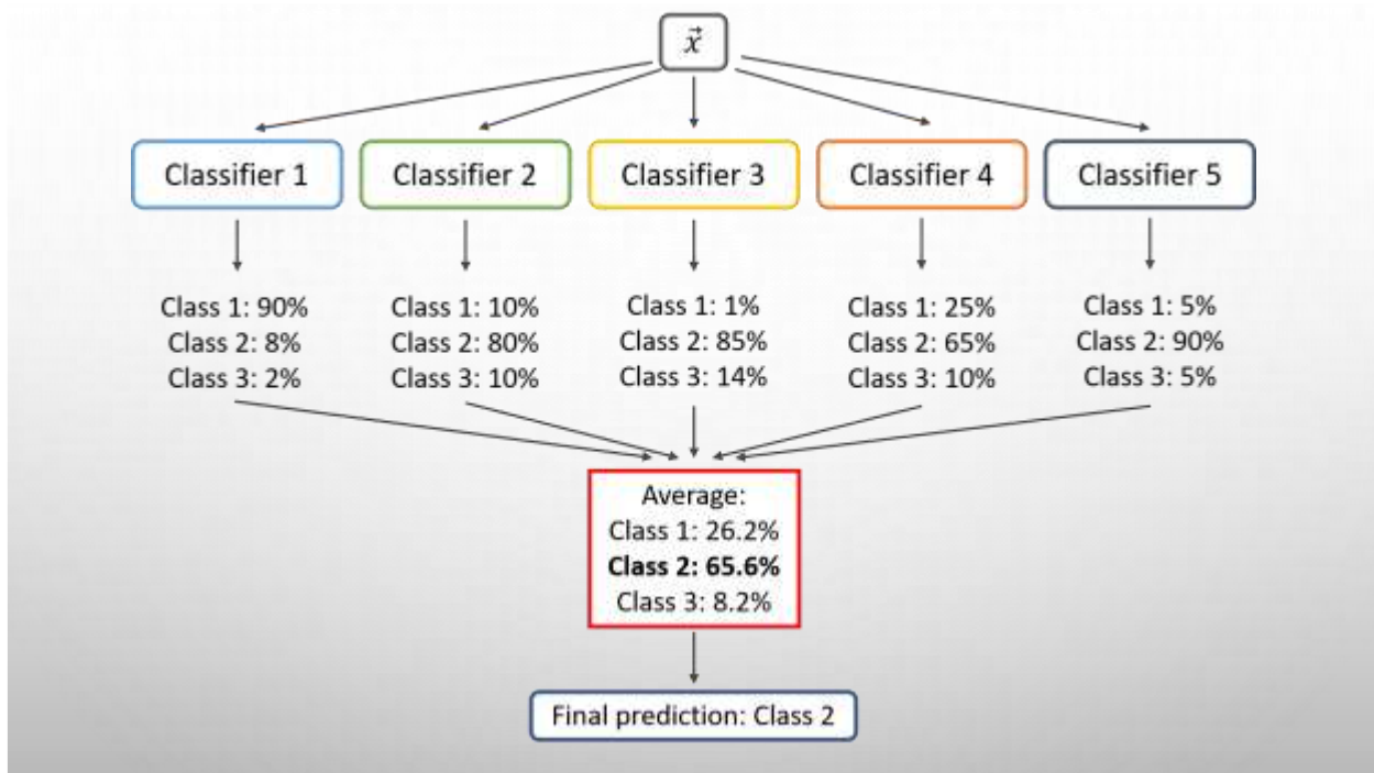
Figure 1: visualization of the concept of voting-based ensemble learning classifier.
