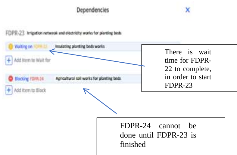
Figure 10: Dependencies window
