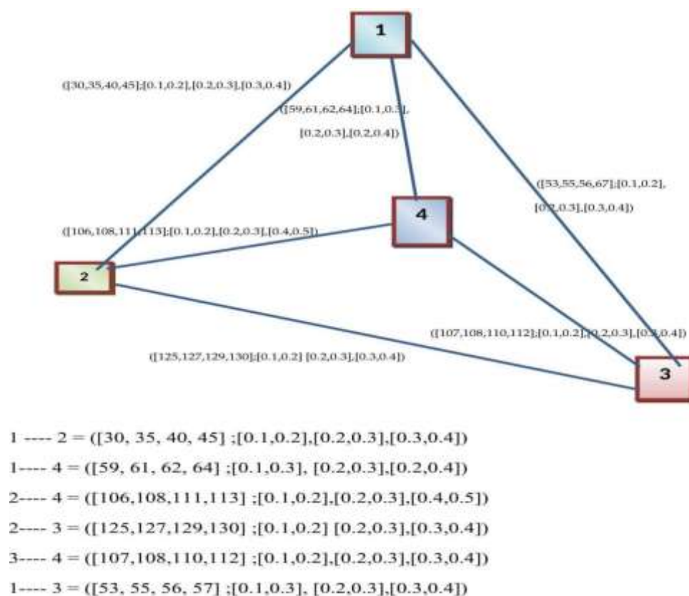
Figure 1: Interval Valued Neutrosophic Fuzzy Shortest Cycle Route Problem.
