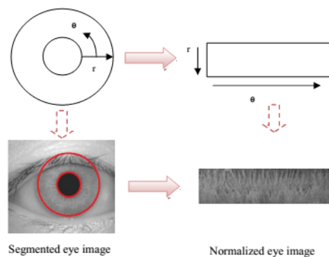
Figure 4: DRS Model
