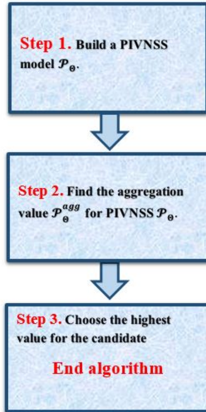
Figure 1: Algorithm
