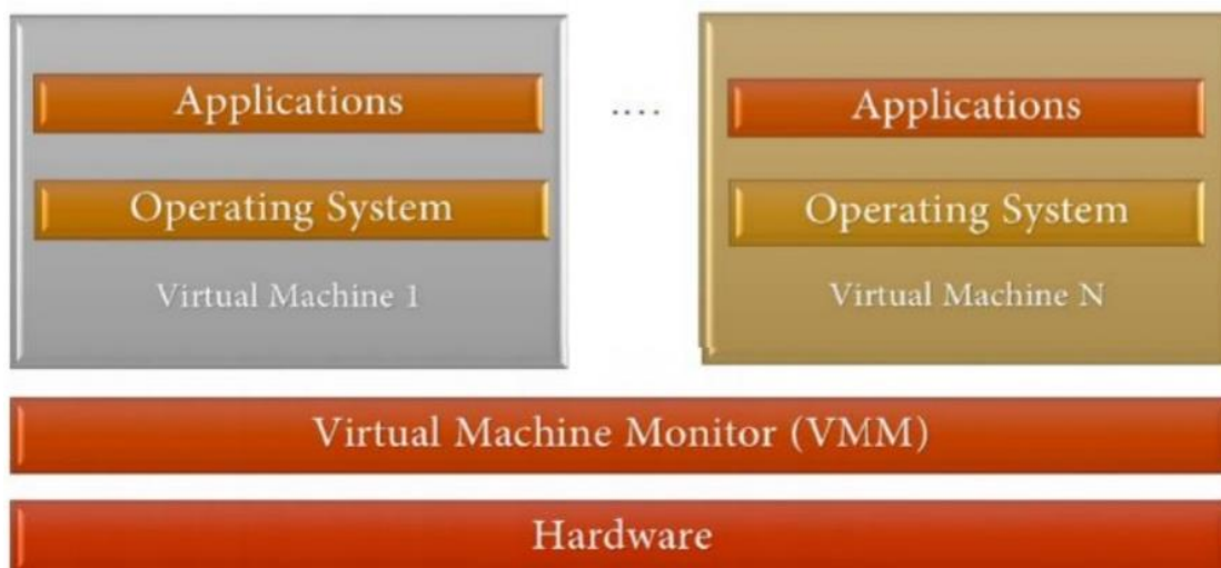
Figure 2: virtual environment
