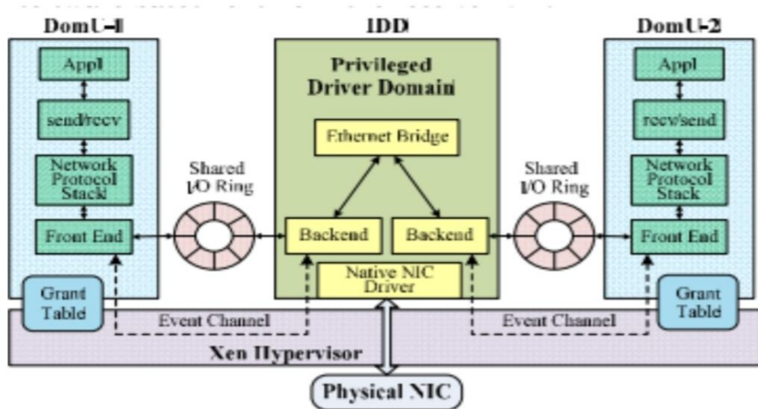
Figure 6: XEN network structure
