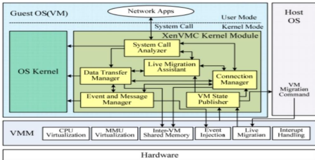
Figure 7: XENVMC kernel module
