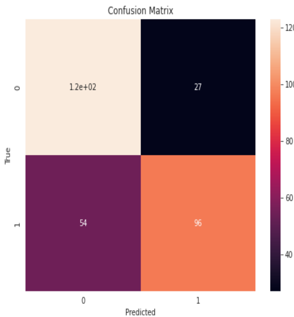
Figure 4: confusion matrix of our autism classifier
