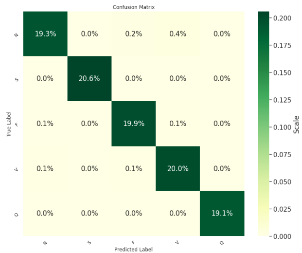
Figure 10: Confusion matrix of ResNet on test set of MIT-BIH data
