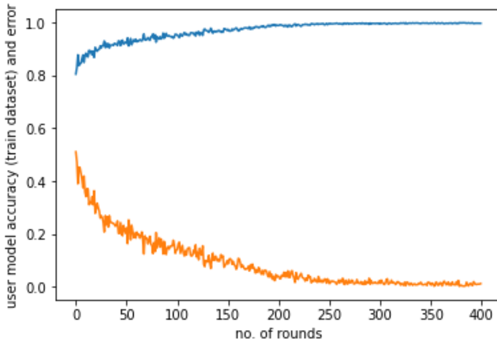
Figure 3: Hacker
